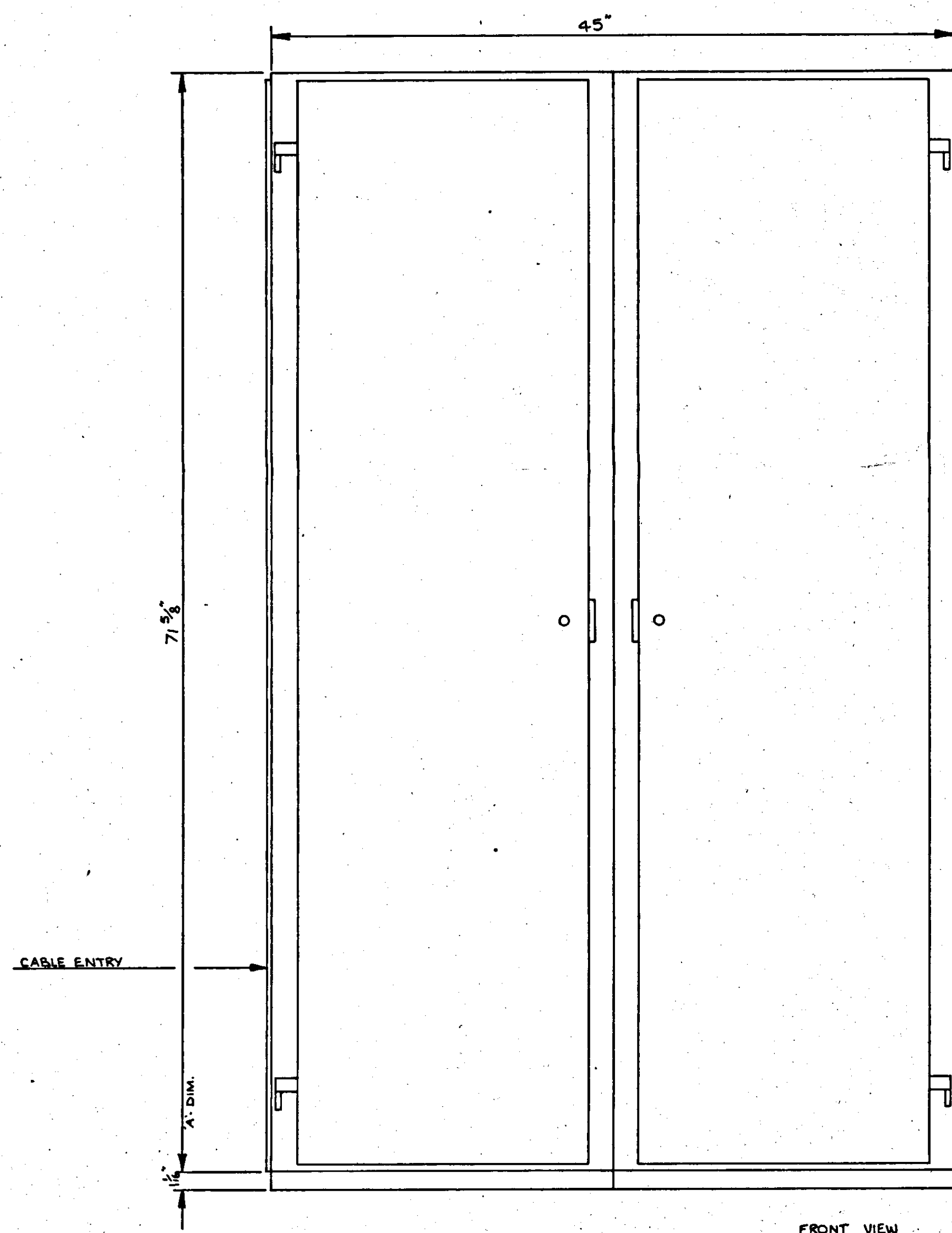
FRONT VIEW
